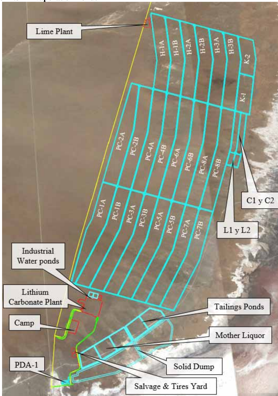
Figure 17.5 Evaporation Ponds
