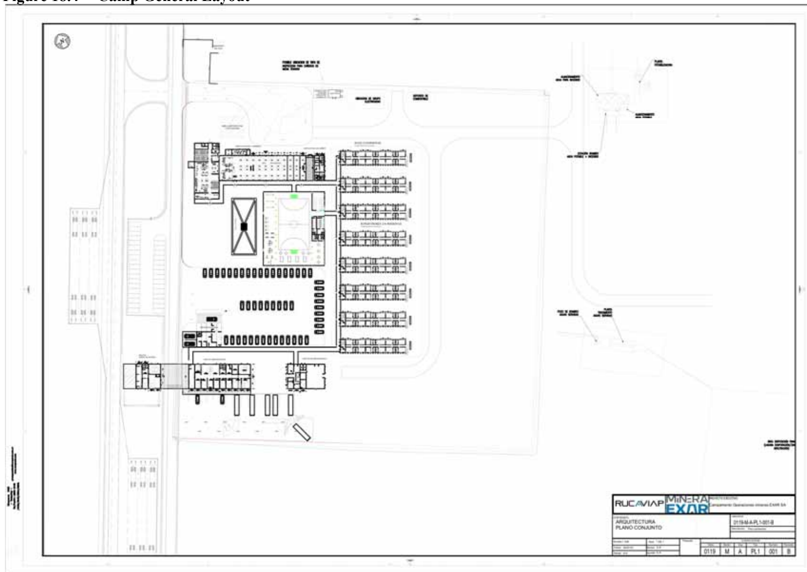
Figure 18.4 Camp General Layout
