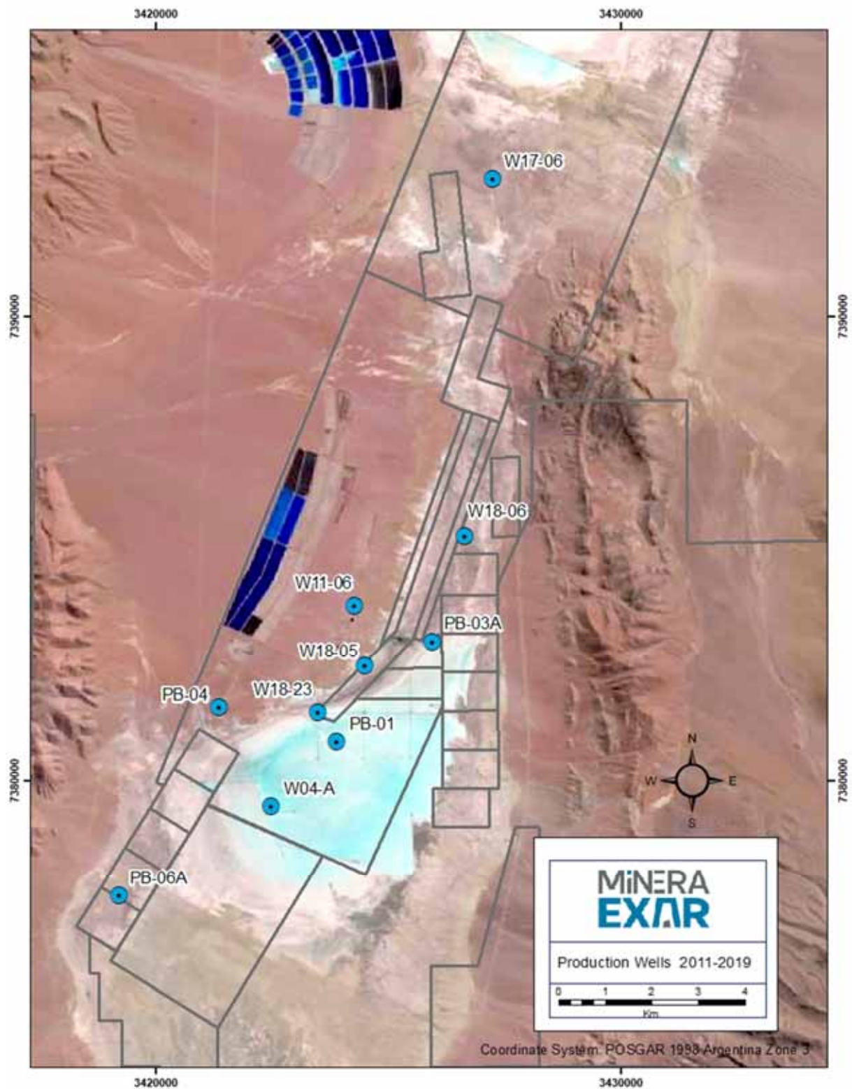
Figure 9.22 Production Wells
