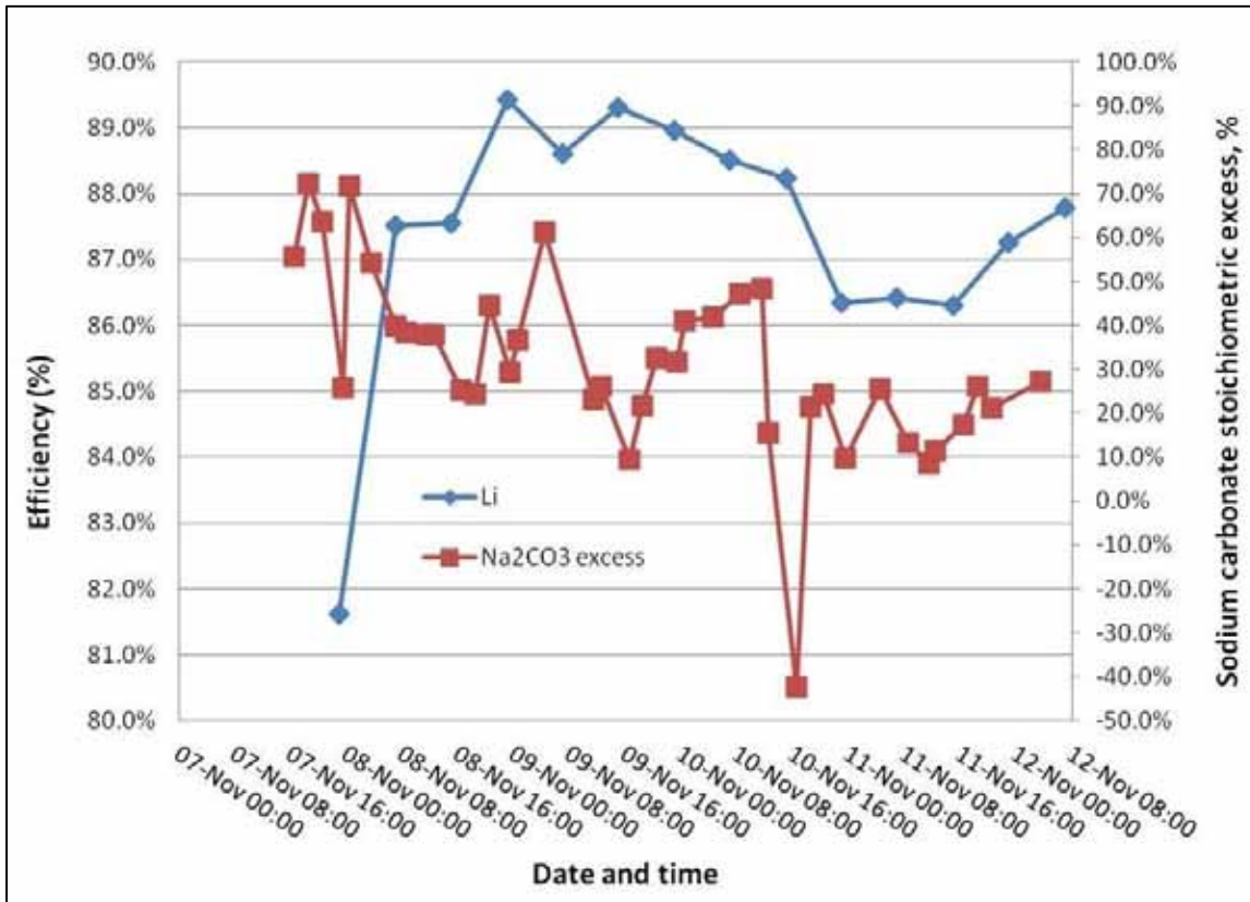
Figure 13.13 Li Precipitation Efficiency
