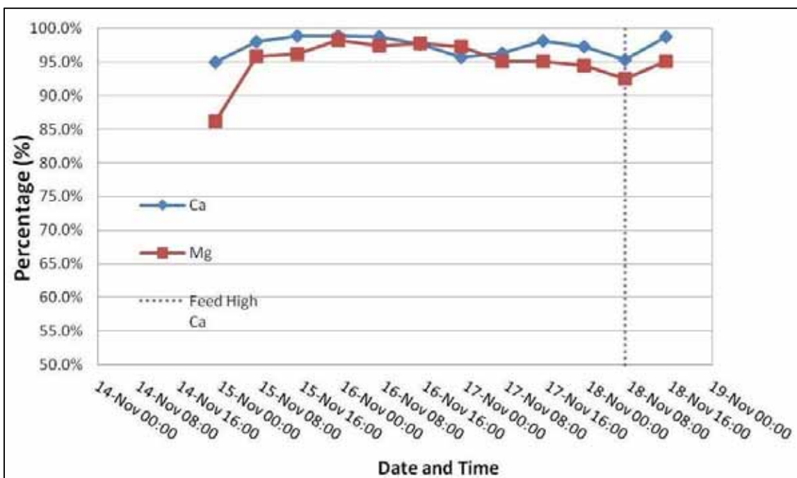
Figure 13.12 Ca and Mg Precipitation Efficiency
