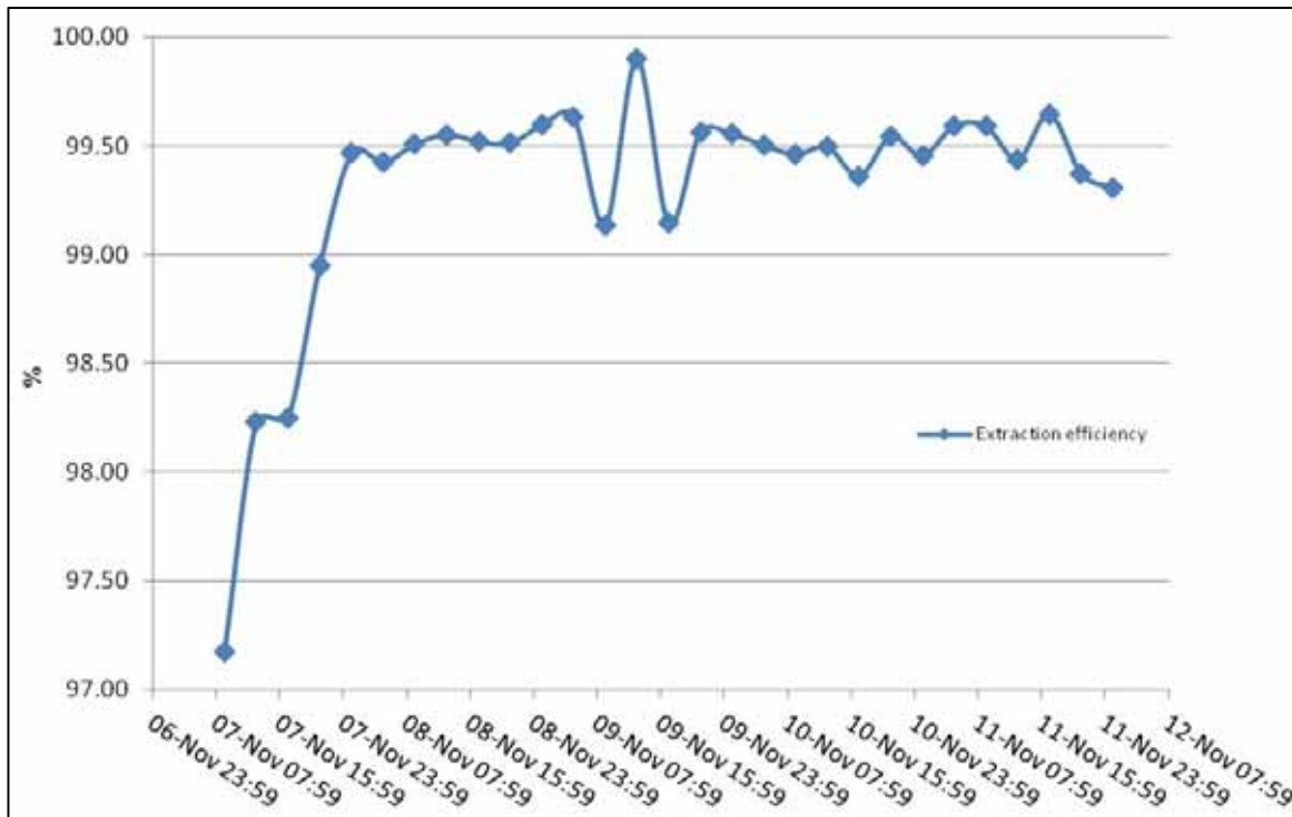
Figure 13.11 SX Process Boron Extraction Efficiency
