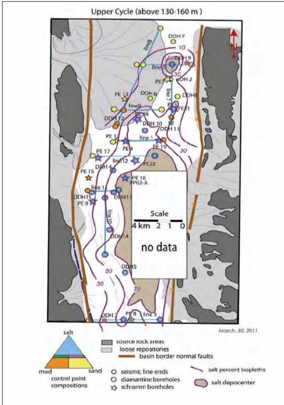
Figure 7.8 Salt Percent Isopleths of the Upper Cycle
