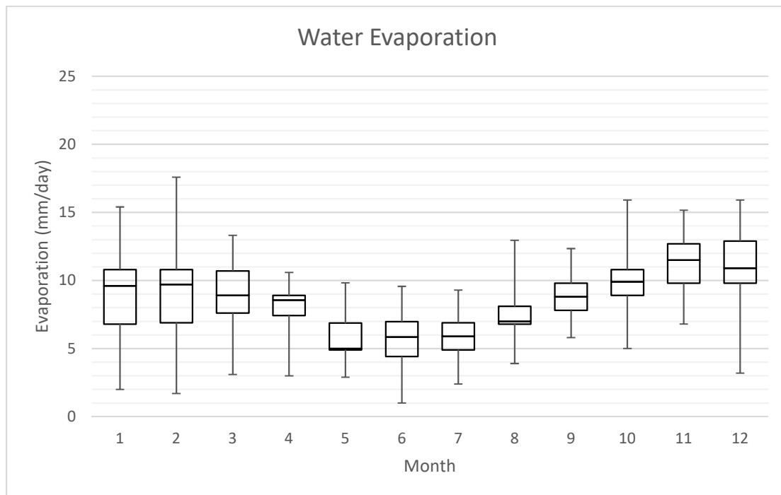
Figure 13.6 Water Evaporation
