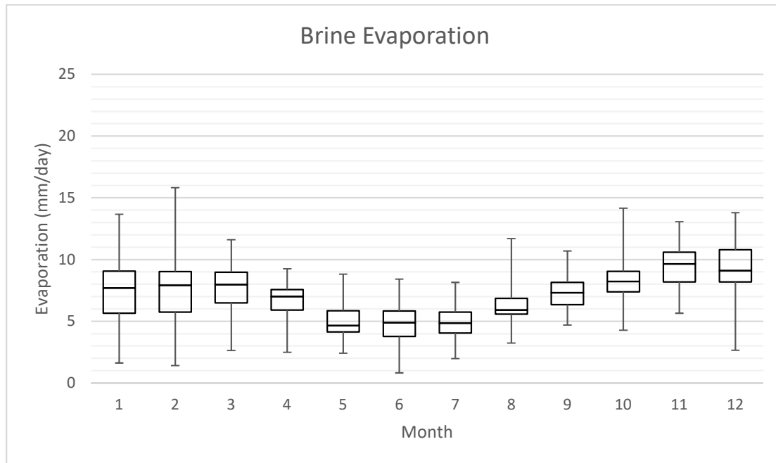
Figure 13.5 Brine Evaporation
