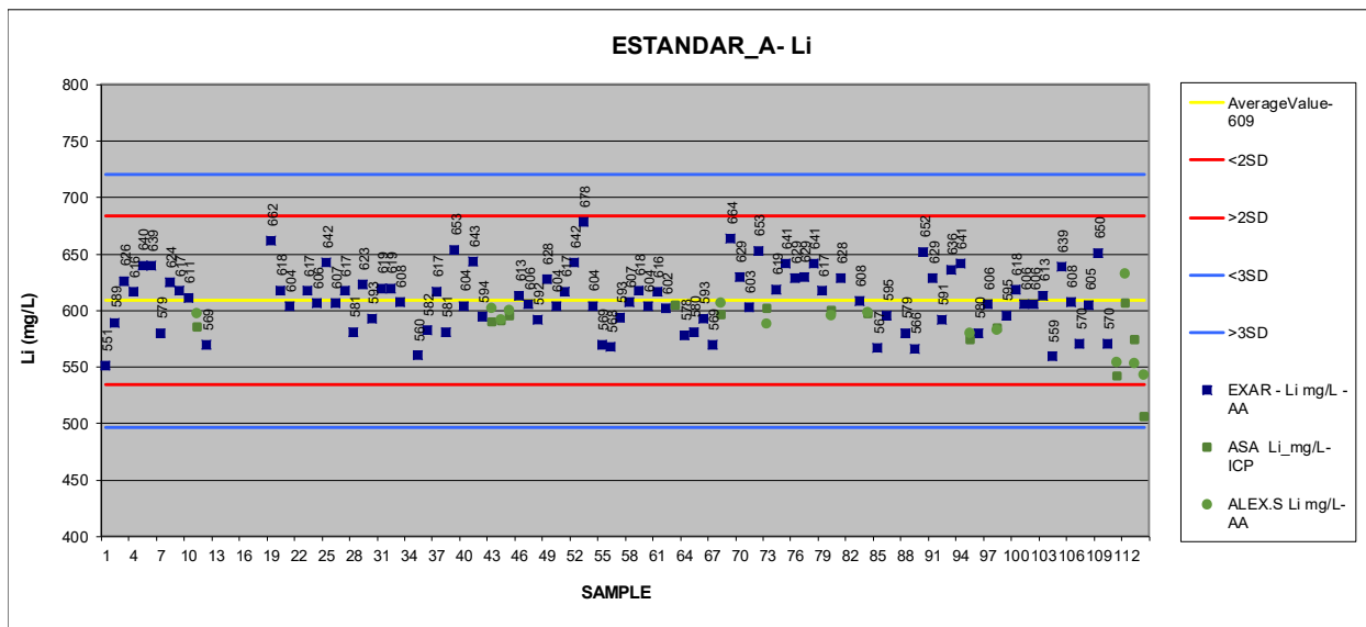
Figure 12.7 Performance of Estandar A
